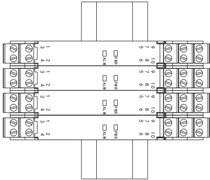
Vertically installation
